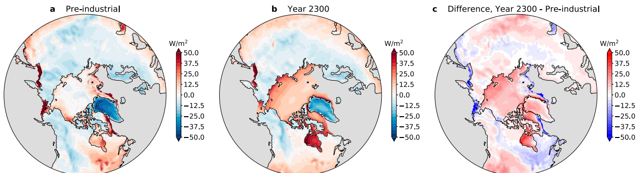
FIG. 3. Changes in surface sensible heat flux with the disappearance of Arctic sea ice. Wintertime climatology over 50 simulated winters of surface sensible heat flux, masked in gray to exclude regions with open ocean in the preindustrial period (both sea ice and land fraction less than 50%). It includes (left) preindustrial model climatology, (center) year 2300, and (right) the difference between the two scenarios. Positive values indicate heat flux from the surface into the atmosphere.
