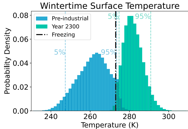
FIG. 1. Narrowing of the wintertime surface temperature distribution in warmer climates. Distribution of hourly 2-m surface air temperature over the interior of North America (see gray dashed box in Fig. 2) between 1 Dec and 28 Feb over 50 simulated winters. The preindustrial scenario is shown in blue, and the year 2300 scenario is shown in green. For reference, the 5th and 95th percentiles are marked by colored dashed lines, and the freezing temperature (273 K) is marked by a black dashed line.
