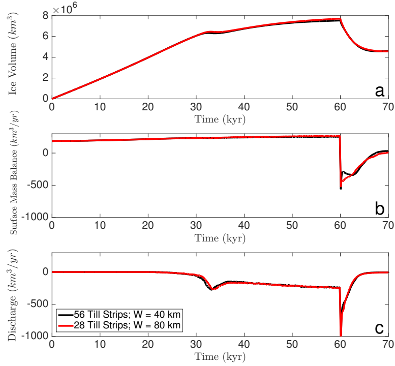
Figure 2. Sensitivity of deglacial ice sheet response to changes in till configuration. Black lines are configured with 56 weak till strips of 40 km width each (same as black line in Figure 2 of main text). Red lines are configured with 28 weak till strips of 80 km width. (a) Ice volume. (b) Surface mass balance. (c) Discharge due to calving at the ice sheet margin following.
