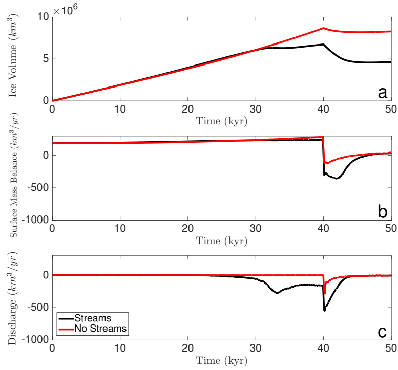
Figure 4. Sensitivity of ice sheet evolution to presence of ice streams. Black lines are configured with ice streams (same as black line in Figure 2 of main text). Red lines are configured with \phi = 80^\circ everywhere in model domain. (a) Ice volume. (b) Surface mass balance. (c) Discharge due to calving at the ice sheet margin following.
