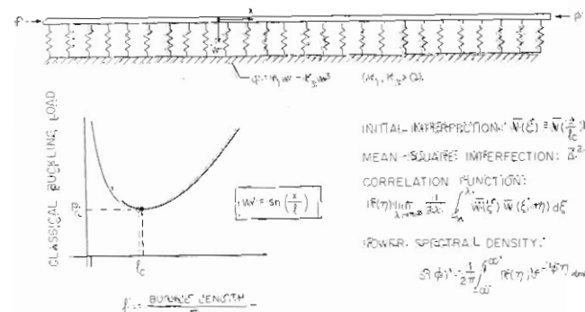
Fig. 7 Infinitely long column with random initial imperfections on a nonlinear foundation.
