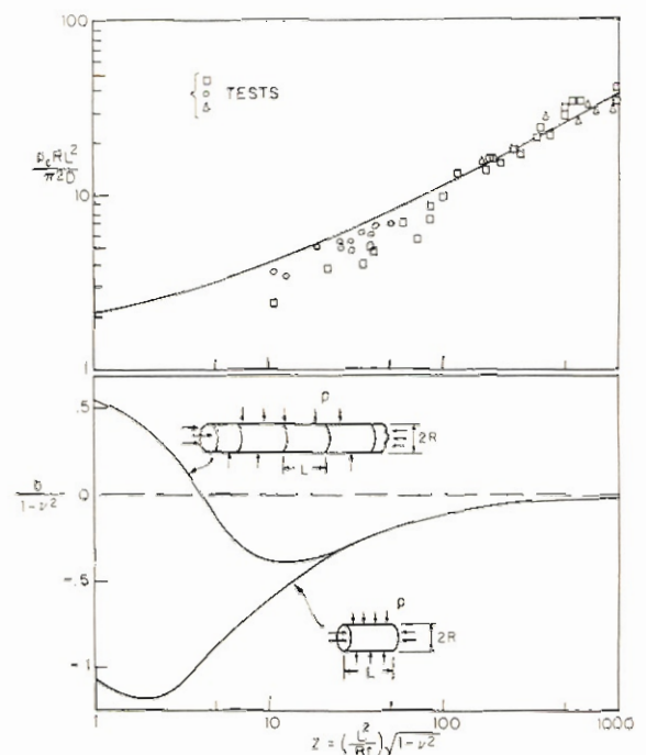
Fig. 3 Classical buckling and imperfection-sensitivity of simply supported cylinders under hydrostatic loading.
