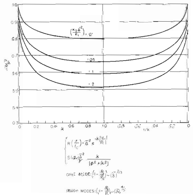
Fig. 8 Buckling loads of column with random imperfections.
