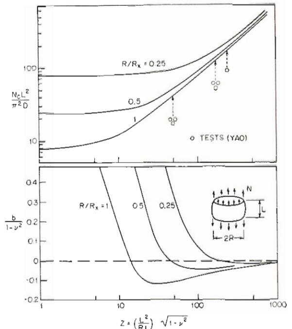
Fig. 5 Classical buckling and imperfection-sensitivity of simply supported toroidal segments under tension.
