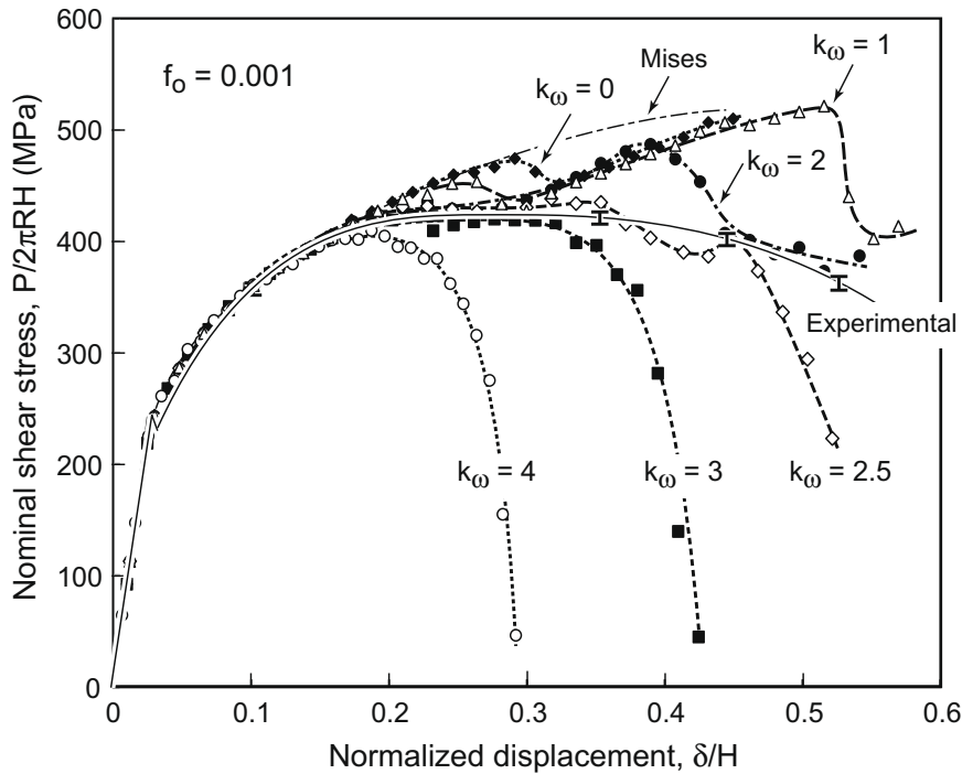
Fig. 10. Measured and computed shear-off response.
