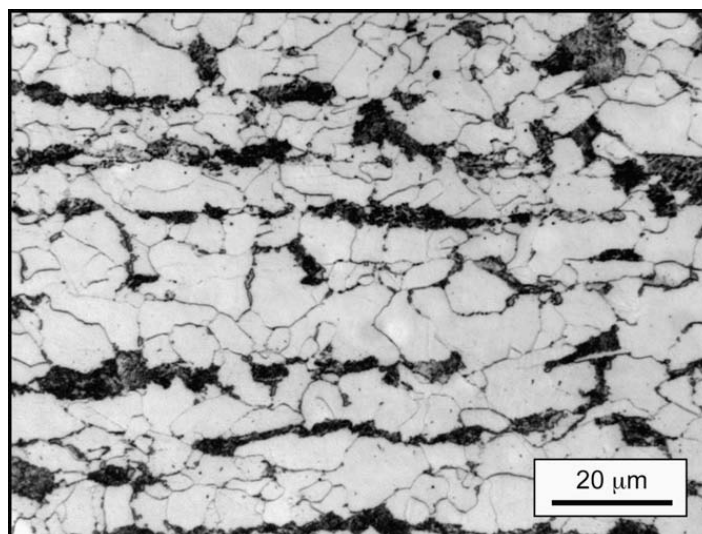
Fig. 1. Optical micrograph of polished and etched cross-section through DH36 steel plate, showing a microstructure of ferrite (light) and pearlite (dark).
