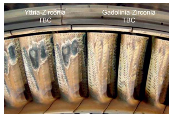
Figure 2. Comparison of typical distress experienced by conventional thermal-barrier coatings (TBCs) based on 7–8% yttria-stabilized zirconia with an advanced TBC based on Gd_xZr_{1-x}O_{2-x/2} pyrochlore, where x \approx 0.5 . The airfoils were part of an engine test in actual aircraft operation. 26 Courtesy of M.J. Maloney, Pratt & Whitney.
