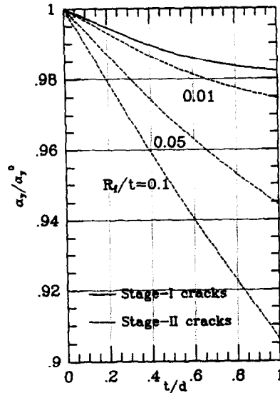
Fig. 11. Effect of fiber radius to half ply thickness ratio R_f/t on the longitudinal CTE of a perfectly bonded cross-ply in the presence of stage-II matrix cracks. The constitutive parameters used are \rho = 0.4 , \nu = 0.2 , E_f/E_m = 2 and \alpha_f/\alpha_m = 0.5 .
