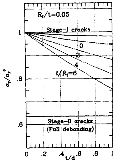
Fig. 12. Effect of frictionless debonding on the longitudinal CTE of a cross-ply laminate with stage-II matrix cracks for R_f/t = 0.05 . The constitutive parameters used are identical to those listed in Fig. 11.
