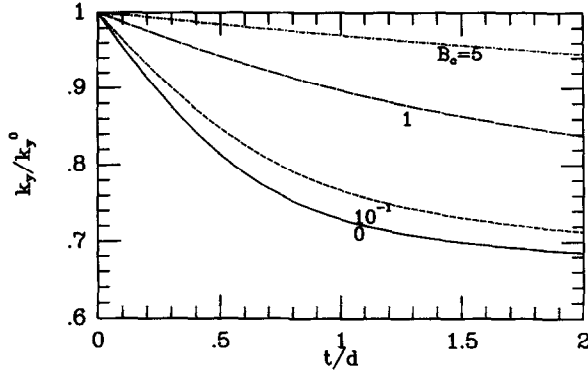
Fig. 5. The effect on the overall longitudinal thermal conductivity of varying the Biot number for Stage-I matrix cracks for k_L/k_T = 2 .
