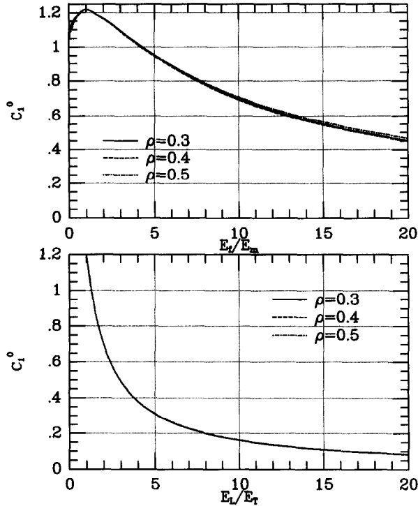
Fig. 8. Numerical results for C_1^0 as function of (a) E_f/E_m ; and (b) E_L/E_T .
